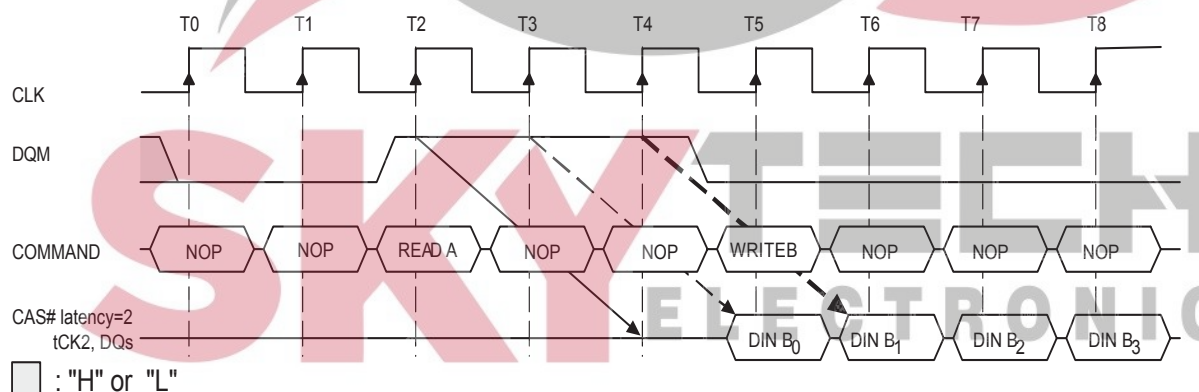
Read to Write Interval (Burst Length = 4, CAS#Latency = 2)
